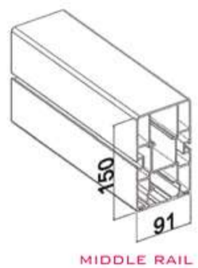
MIDDLE RAIL
